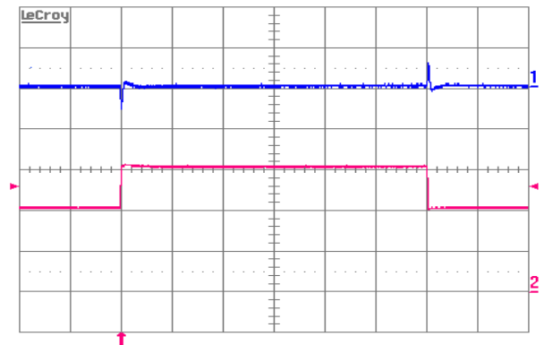
Figure 9. Output voltage response to load current step-change (20 A – 30 A – 20 A) at V_{in} = 48\text{ V} . Top trace: output voltage (100 mV/div.). Bottom trace: load current (10 A/div.). Current slew rate: 2.5 A/ \mu\text{s} . C_o = 470\text{ }\mu\text{F POS} + 1\text{ }\mu\text{F} ceramic. Time scale: 0.2 ms/div.
